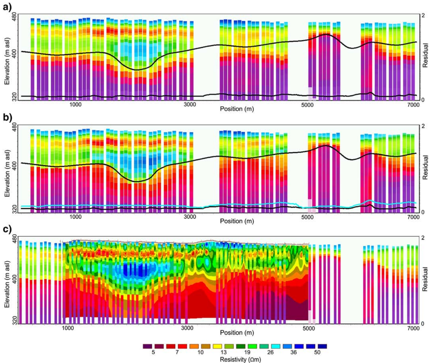
Fig. 6. S2007 calibrated VTEM inversion results. (a) Calibrated and unconstrained. Upper solid black line is the bedrock reflection surface. Lower solid black line is the unconstrained data residual or misfit. (b) Calibrated and constrained with bedrock reflection surface. Solid blue line is the constrained data residual. (c) Comparison of ERT model with the calibrated and constrained VTEM model showing significantly improved agreement. (For interpretation of the references to colour in this figure, the reader is referred to the web version of this article.)
