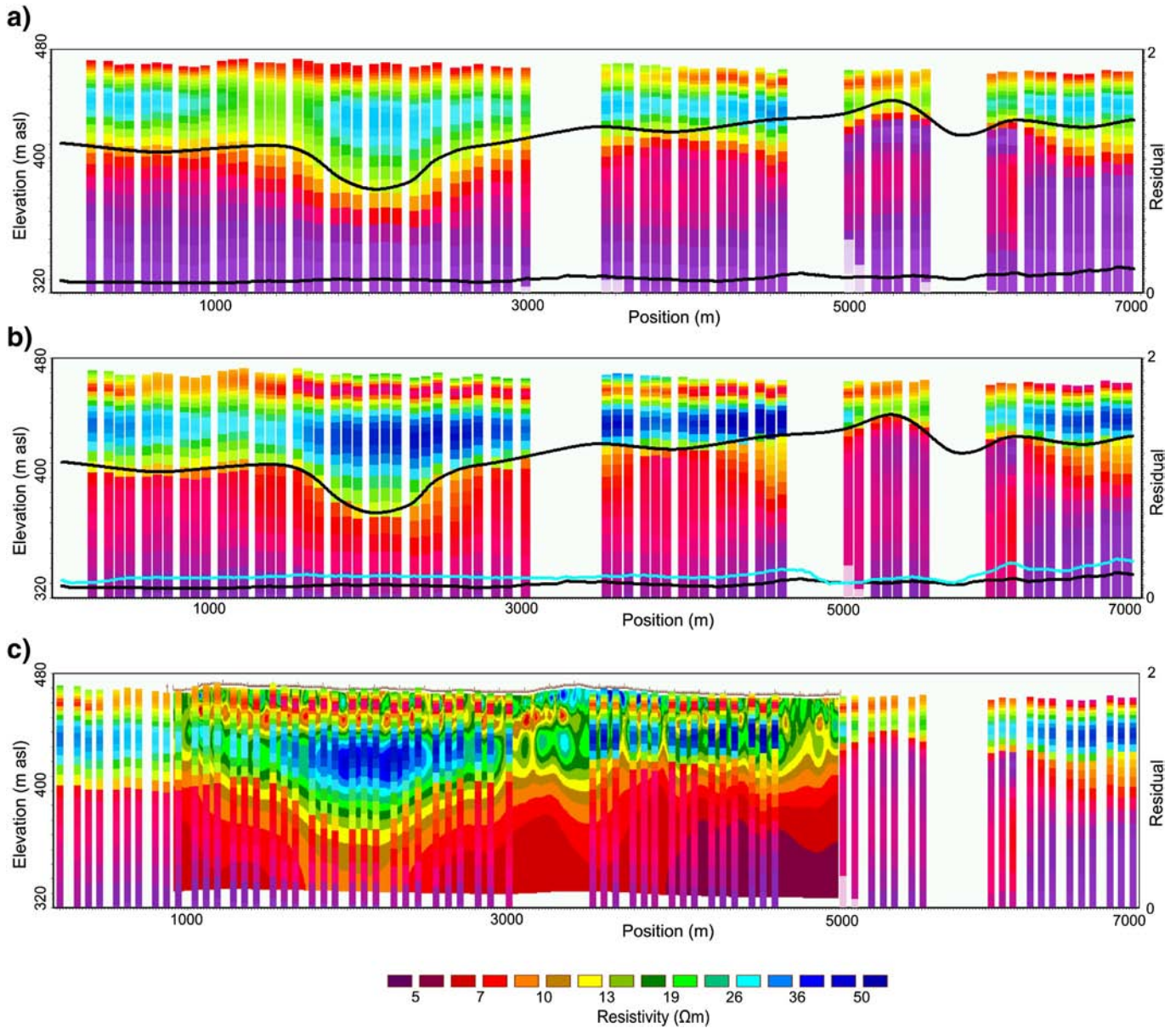
Fig. 4. S2007 VTEM inversion results. (a) Unconstrained. Upper solid black line is the bedrock reflection surface. Lower solid black line is the unconstrained data residual or misfit. (b) Constrained with bedrock reflection surface and bedrock conductivity of 7 \Omega\text{m} (standard deviation factor of 1.5). Solid blue line is the constrained data residual. (c) Comparison of ERT model with the constrained VTEM model. The VTEM model underestimates the depth to the shallow conductive layer by approximately 10 m. (For interpretation of the references to colour in this figure, the reader is referred to the web version of this article.)
